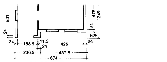
2 Dimensions given around the drawing (drawn at 1:100 cm; units = cm)
